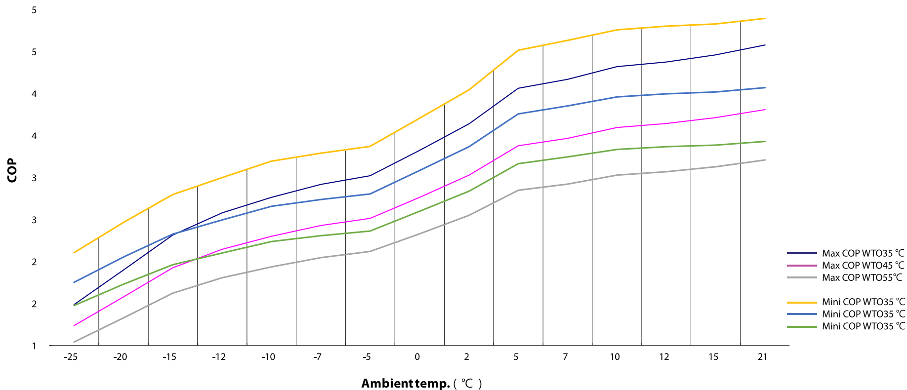
Curve of COP Performance
