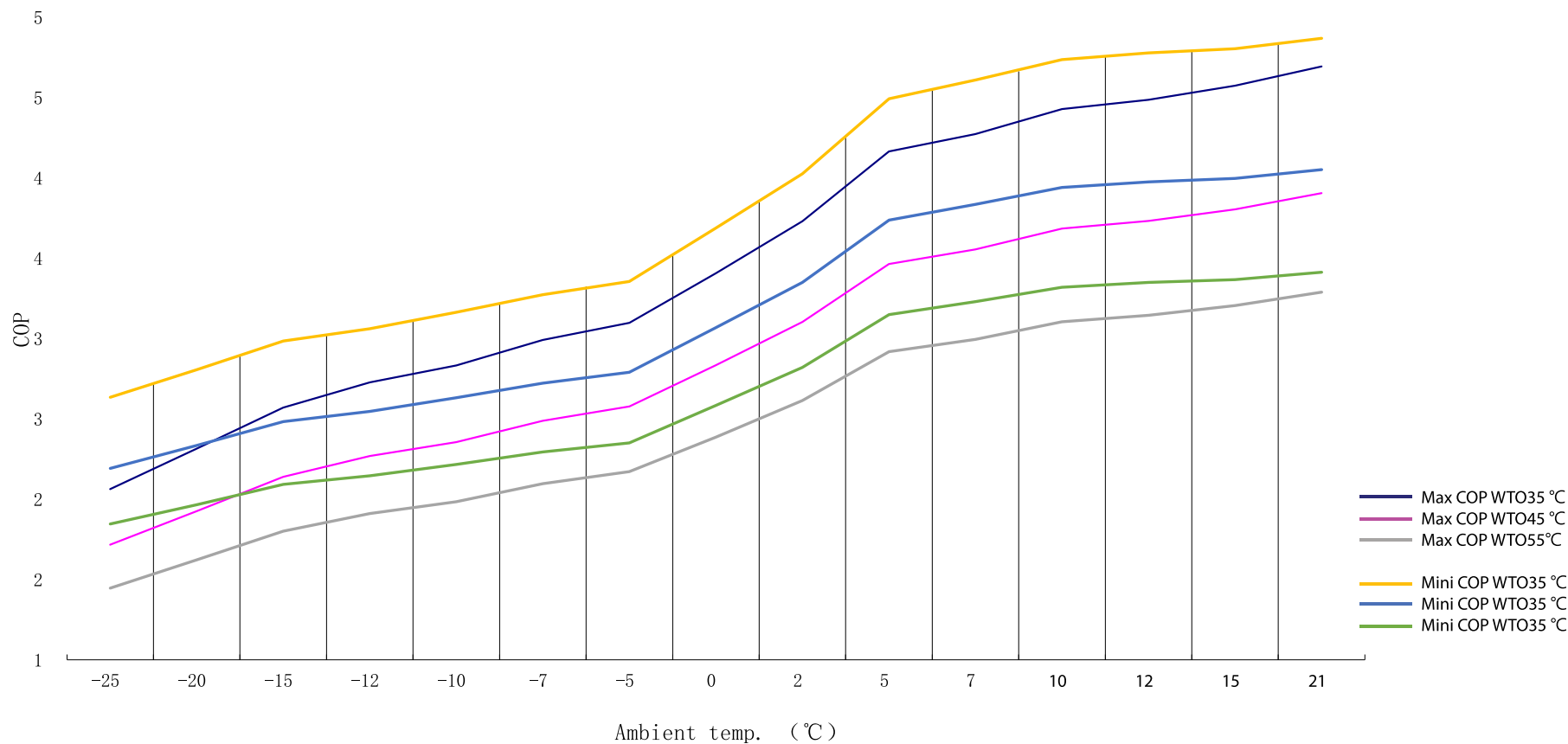
BLP18P3V1MR32 Curve of COP Performance
