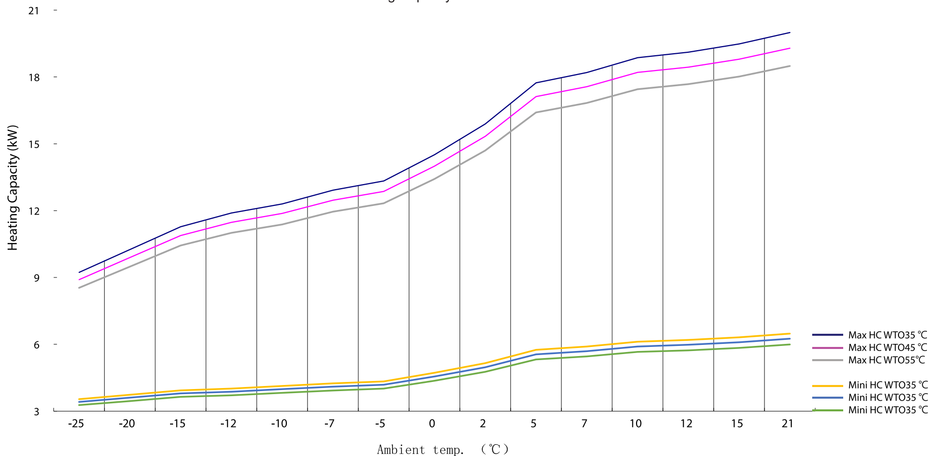
BLP18P3V1MR32 Curve of Heating Capacity Performance
